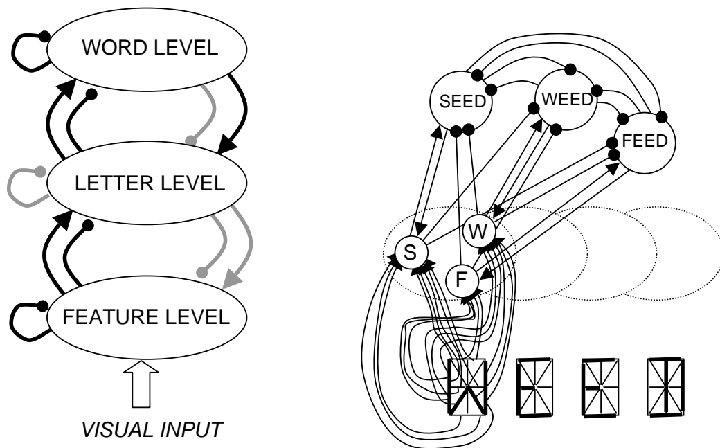
Figure 2. Interactive Activation model of context effects in letter recognition (McClelland & Rumelhart, 1981, 1982). Pointed arrows are excitatory connections, circular headed arrows are inhibitory connections. Left: macro view (connections in gray were set to zero in implemented model). Right: micro view for the connections from the feature level to the first letter position for the letters S, W, and F (only excitatory connections shown) and from the first letter position to the word units SEED, WEED, and FEED (all connections shown).
