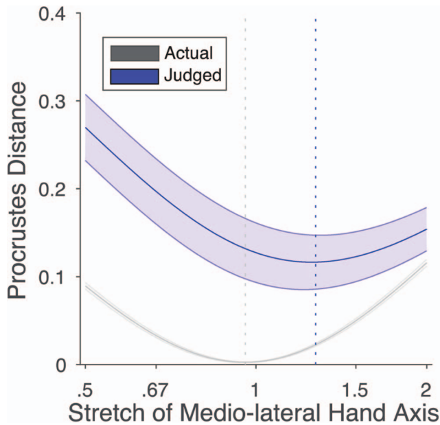
Figure 5. Mean Procrustes distance between actual (light gray) and perceptual (blue/dark gray) maps and idealized grids stretched by different amounts. A stretch of 1 indicates a square grid; stretches greater than 1 indicate stretch in the medio-lateral axis, while stretches less than 1 indicate stretch in the proximo-distal axis. The shaded regions indicate one standard error of the mean. The dotted vertical lines indicate the mean of the best-fitting stretches for perceptual maps (blue/dark gray) and actual maps (light gray). The stretch that minimized the Procrustes distance was substantially larger than 1. Thus, there was clear evidence for stretch in the medio-lateral hand axis for perceptual maps. See the online article for the color version of this figure.
