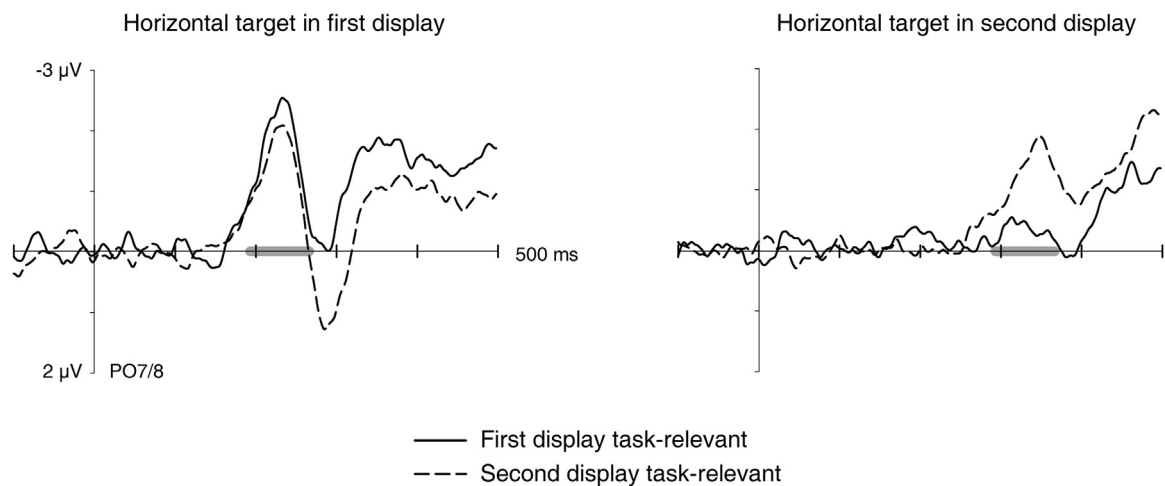
Fig. 4. N2pc results obtained in the horizontal/vertical presentation condition of Experiment 1 . Grand-average ERP waveforms measured in the 500 ms interval after the onset of the first display at posterior electrodes PO7/PO8 contralateral and ipsilateral to the side of the horizontal target-colour item are shown for trials where this item was presented in the first (H1 trials; left panels) or second display (H2 trials; right panels), separately for blocks where the first (D1 blocks; top panels) or second (D2 blocks; middle panels) target-colour item was response-relevant. Bottom panels show the corresponding N2pc difference waves obtained by subtracting ipsilateral from contralateral ERPs, separately for H1 and H2 targets in D1 and D2 blocks. The grey bars on the x-axes represent the respective N2pc time windows.
